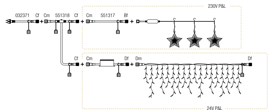
EXAMPLE OF MIXED 230V AND 24V WIRING
